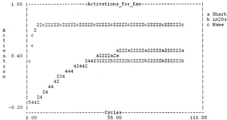
FIGURE 1. The graph showing the activation of the Sharks , in20s , and Ken units, from the file jets.clx , based on a run of the iac program with external input supplied to the Ken unit.
